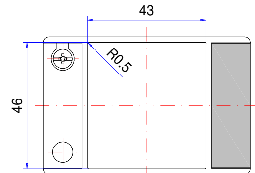
Folie/ Keypad 45.4 +0 -0.2 x 42.4 +0 -0.2
